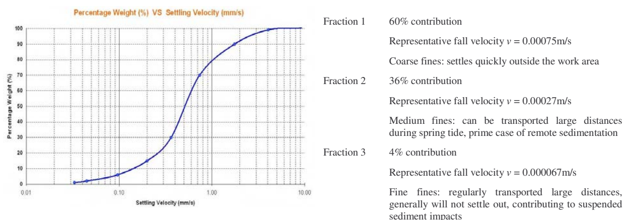
Figure 7. Example sediment fall velocity distribution from Owen Tube test of fine material content of reclamation fill.
