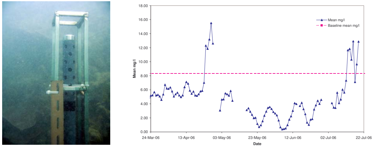
Figure 11. Left: deployed YSI turbidity sensor. Right: time series of turbidity measurements.
