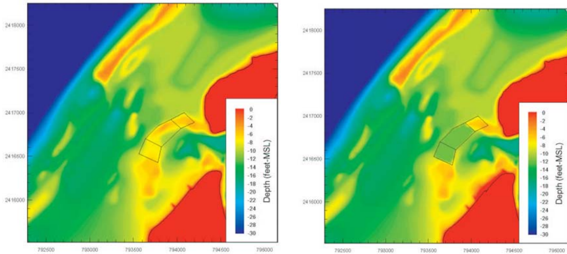
Figure 10. Before Dredge Survey (left) and After Dredge Modeled Bathymetry (right)
