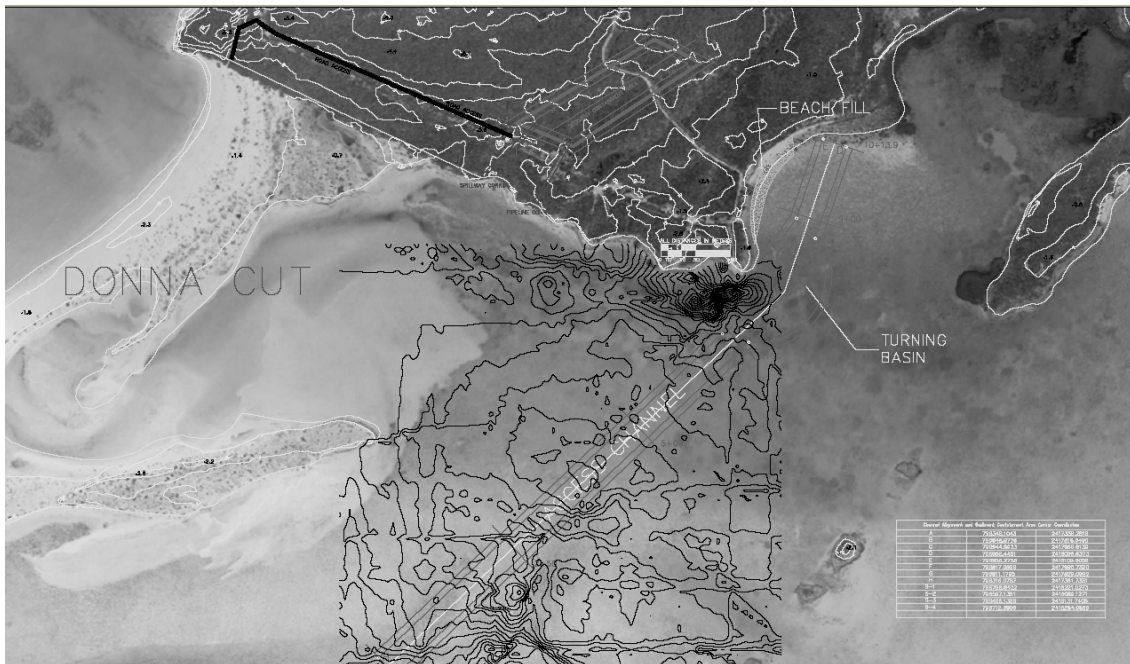
Figure 14. Water Cay Project Layout showing Channel alignment and Bathymetry
