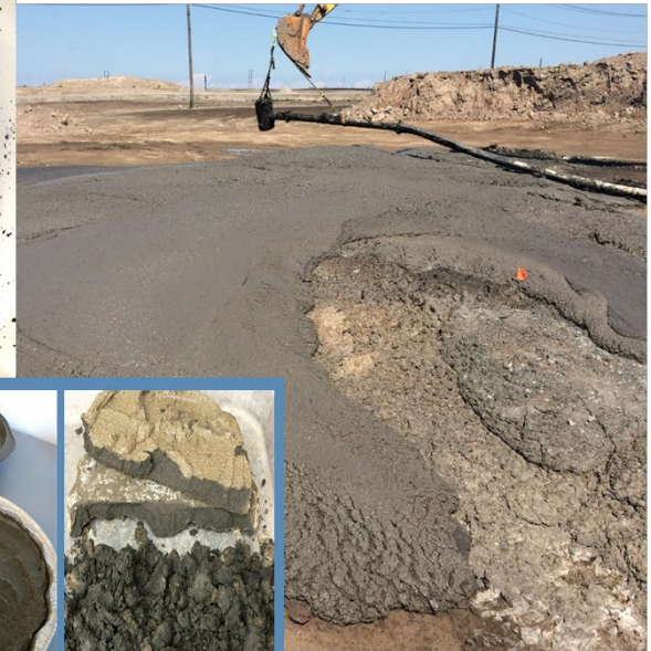
Freshly-placed PDM (8% Portland cement via Pneumatic Flow Tube Mixing)
